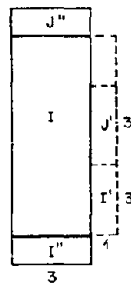
1.c TYPICAL LAYOUT FOR THREE SIDES OF ENTRY HATCH. TOTAL REQUIRED = 3 SHEETS USE PIECES I' AND J' IN POSITION I'' AND J'', FOURTH SIDE REQUIRES A PIECE 3 ft X 4 ft 2 in. WHICH MUST BE CUT FROM THE 17th PIECE OF PLYWOOD. SAVE THE SCRAP TO USE IN CONJUNCTION WITH THE K.A.P.
